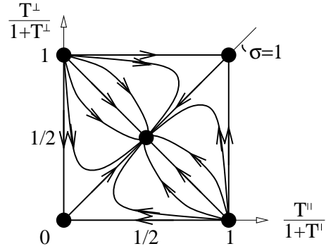
Fig. 1. Equilibrium (center) and non-equilibrium (corners) fixed points of the non-equilibrium SSS model with dynamical anisotropy in the [T^{\parallel}/(1+T^{\parallel}), T^{\perp}/(1+T^{\perp})] -plane.
